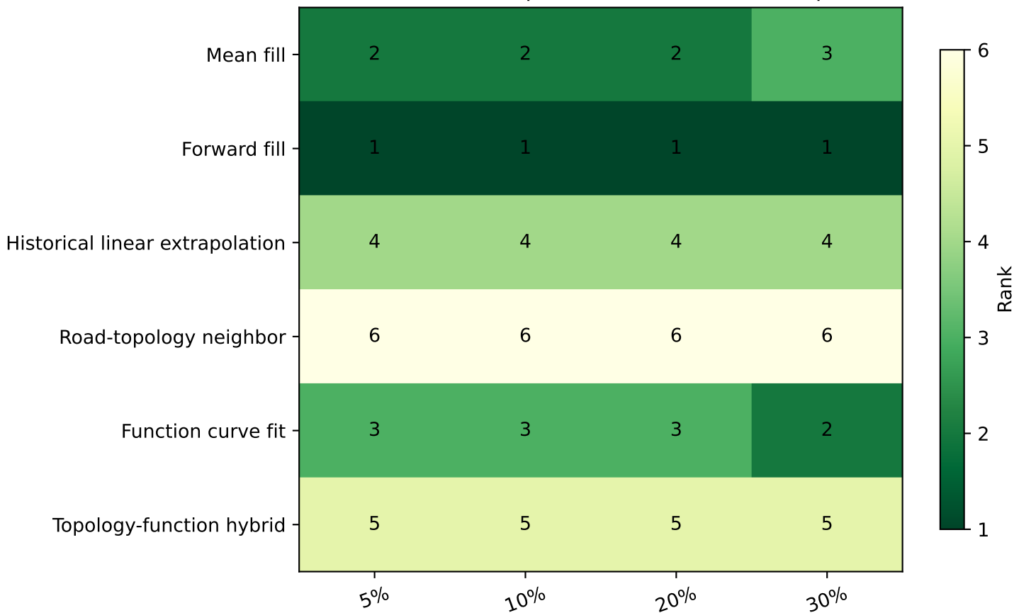
Global MCAR point RMSE Rank Heatmap
