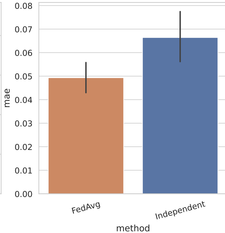
Method Comparison: MAE
