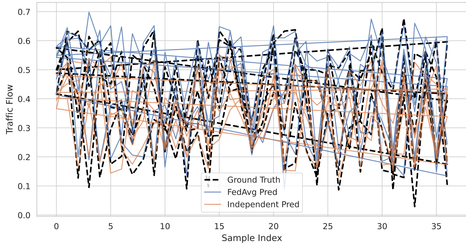
Traffic Flow Prediction Comparison (Client 0)
