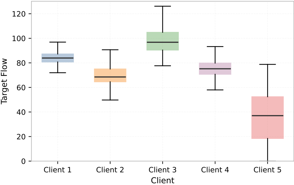
(c) Target-flow Distribution Shift
