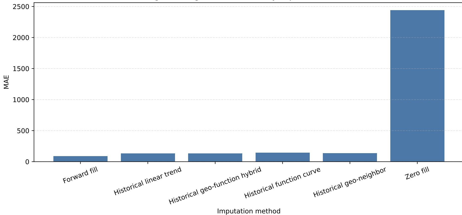
Single missing rate = 5%: MAE by imputation method
