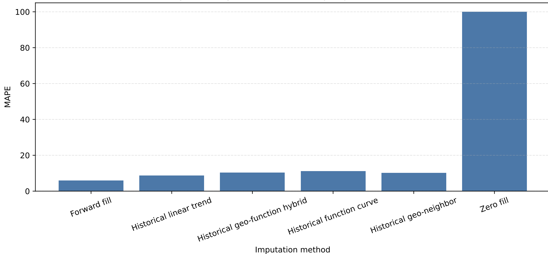
Single missing rate = 5%: MAPE by imputation method
