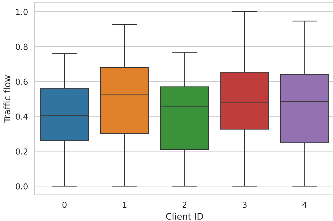
Non-IID traffic distribution by client
