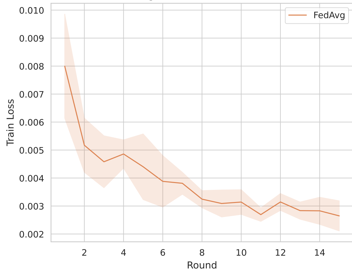
Convergence Mean \pm Std: Train Loss
