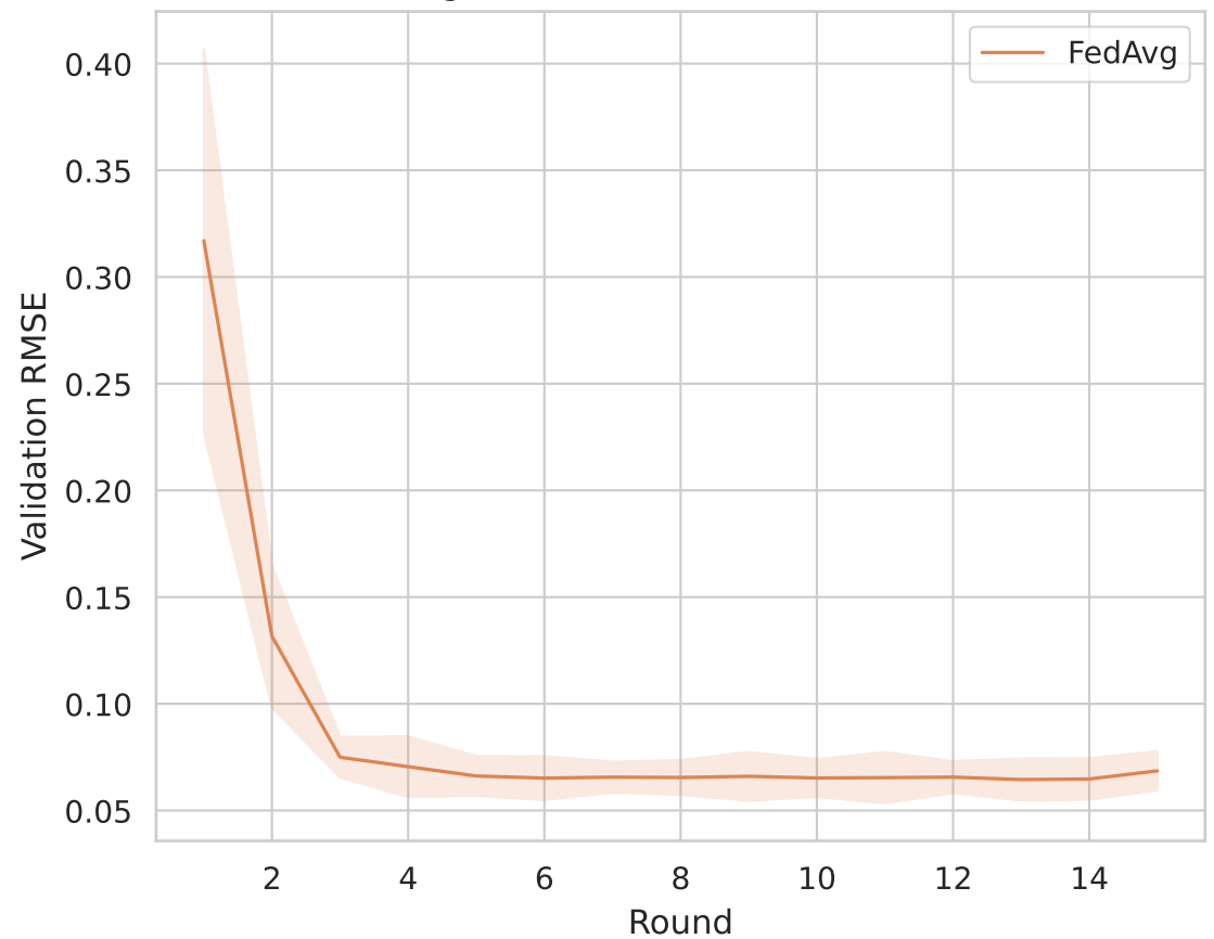
Convergence Mean \pm Std: Validation RMSE
