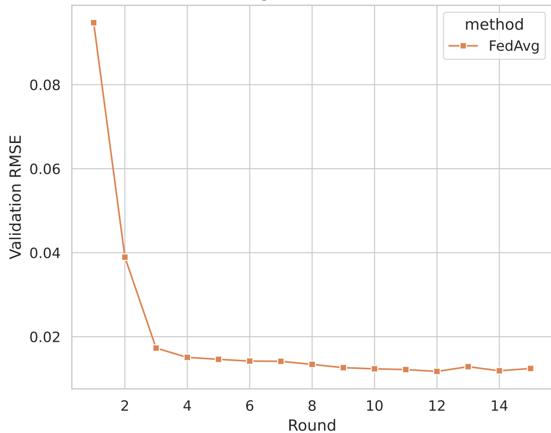
Average Validation RMSE
