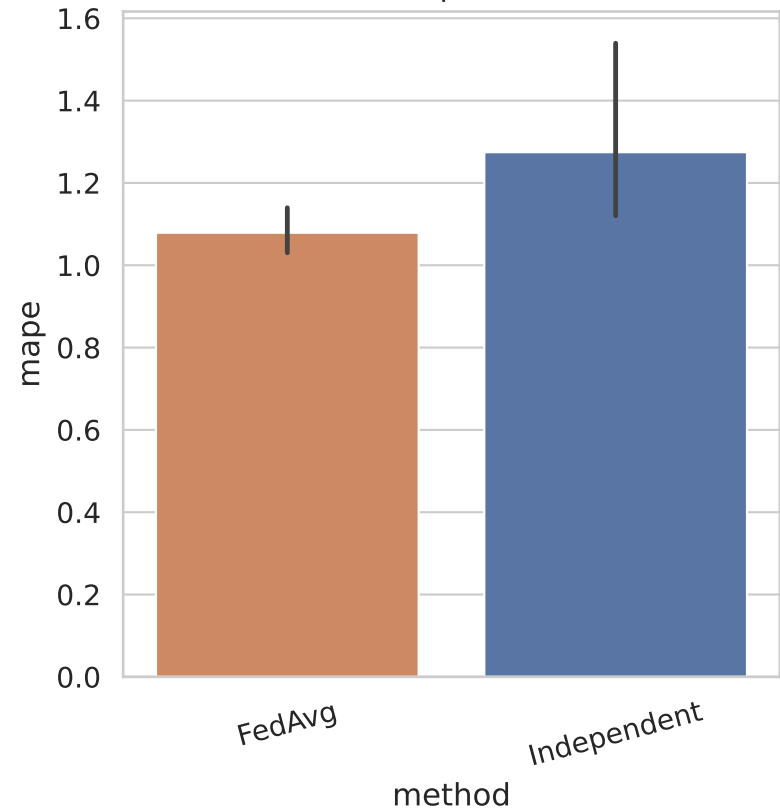
Method Comparison: MAPE
