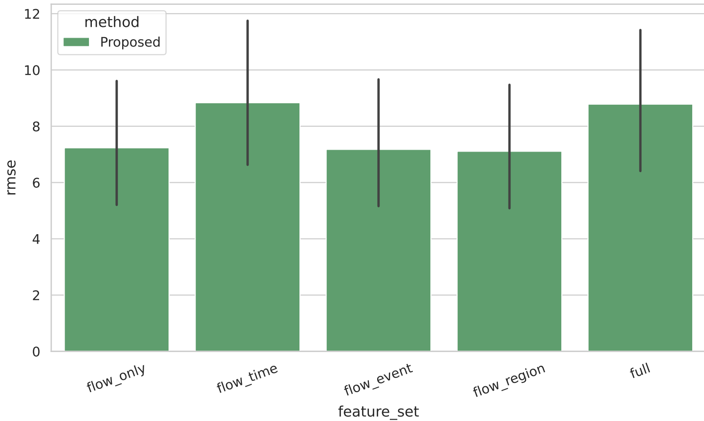
Feature Ablation
