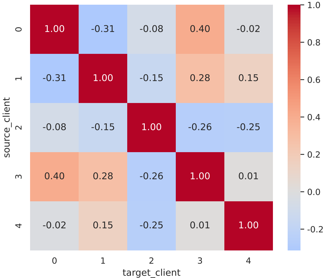
Client Correlation Matrix
