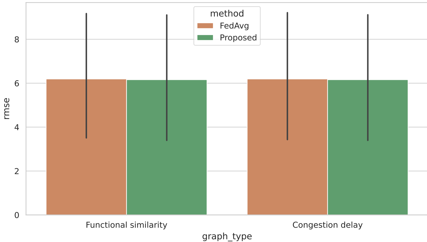
Congestion Delay Training Comparison
