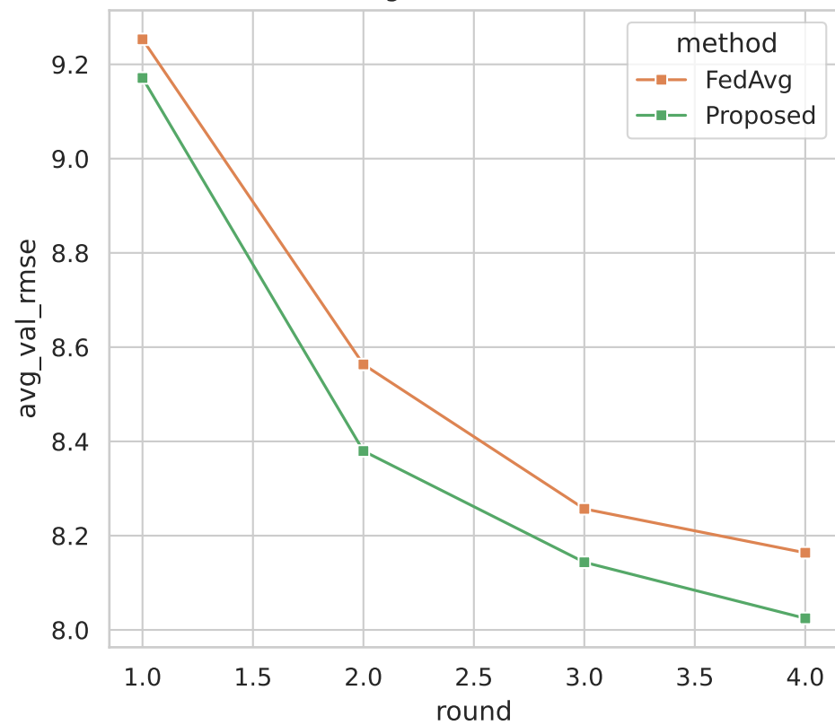
Average Validation RMSE
