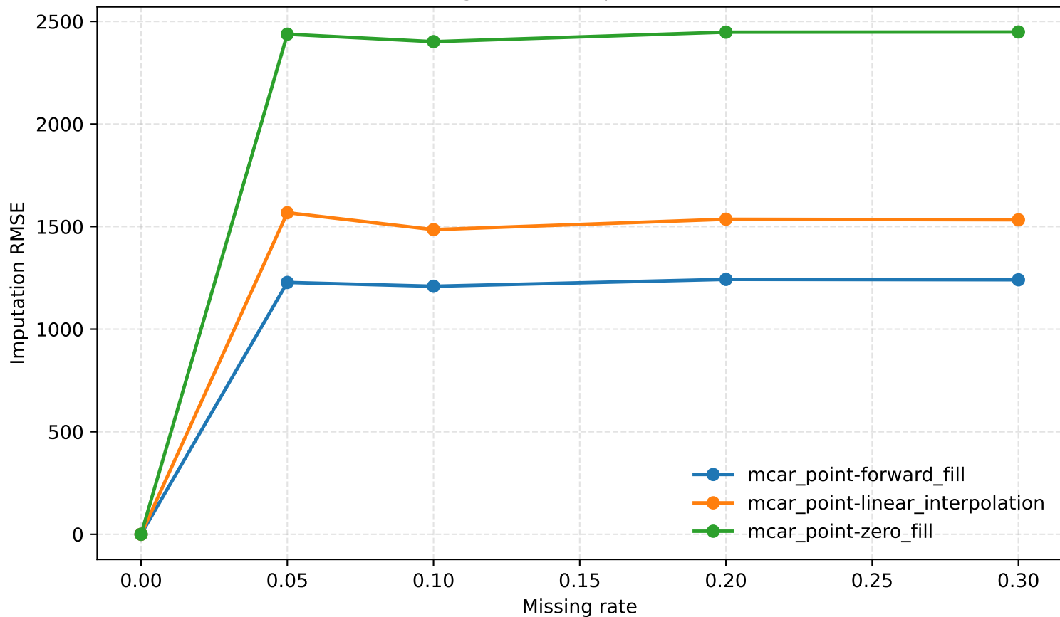
Missing Rate vs Imputation RMSE
