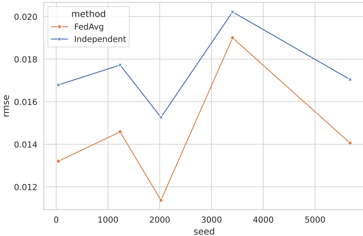
Per-seed RMSE Comparison
