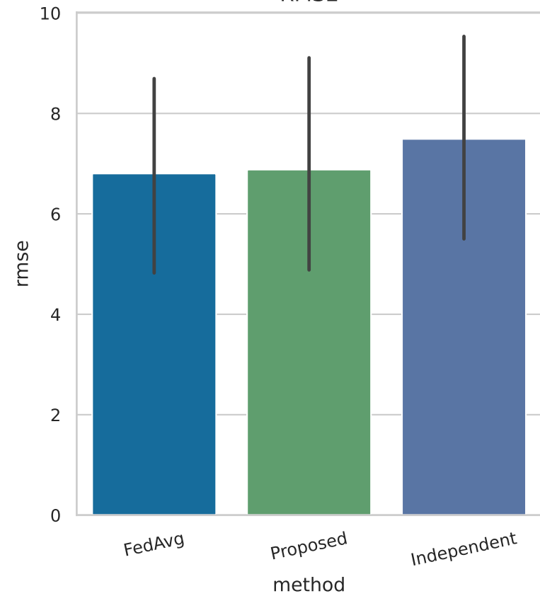
RMSE
