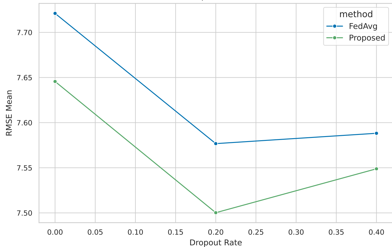
Client Dropout Robustness
