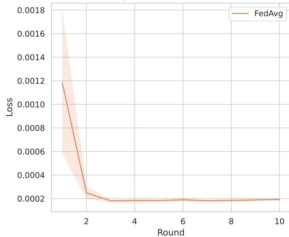
Convergence Mean \pm Std: Train Loss
