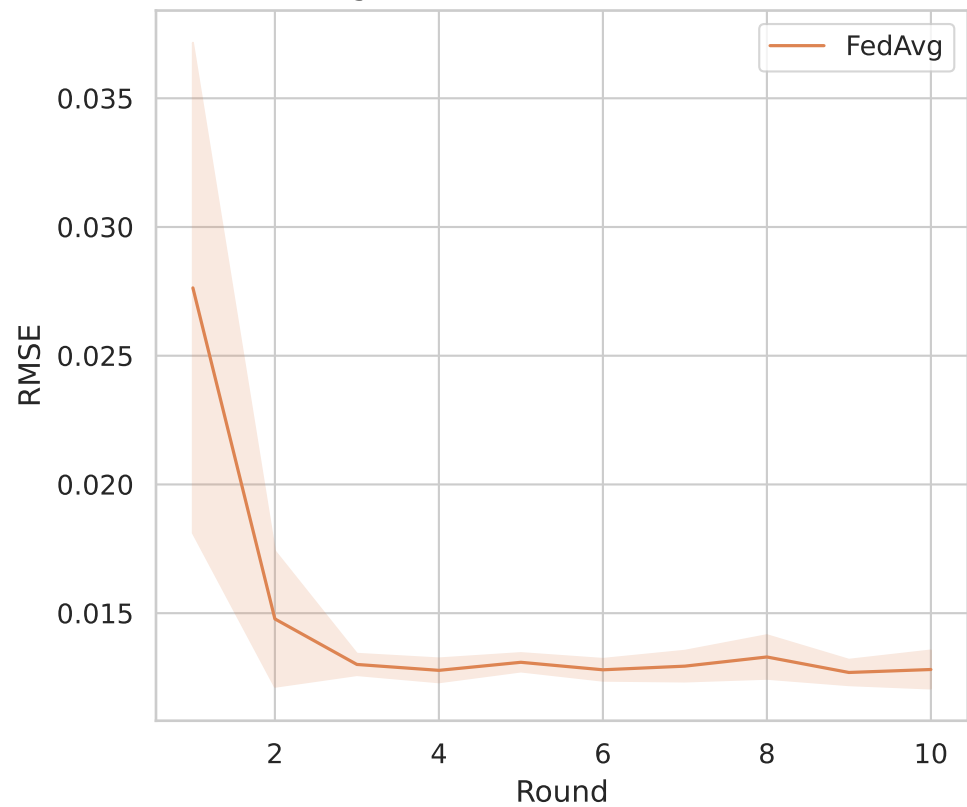
Convergence Mean \pm Std: Validation RMSE
