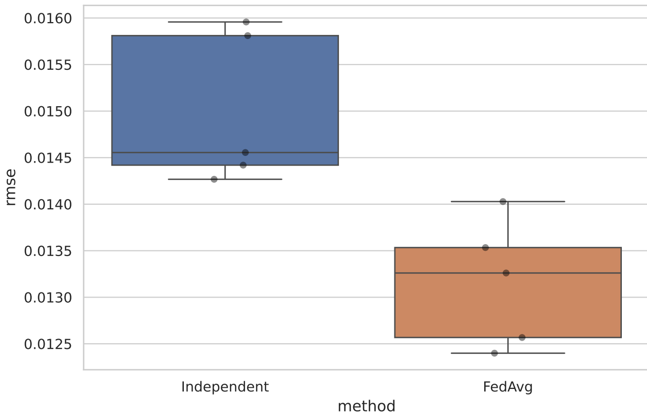
Multi-seed RMSE Distribution
