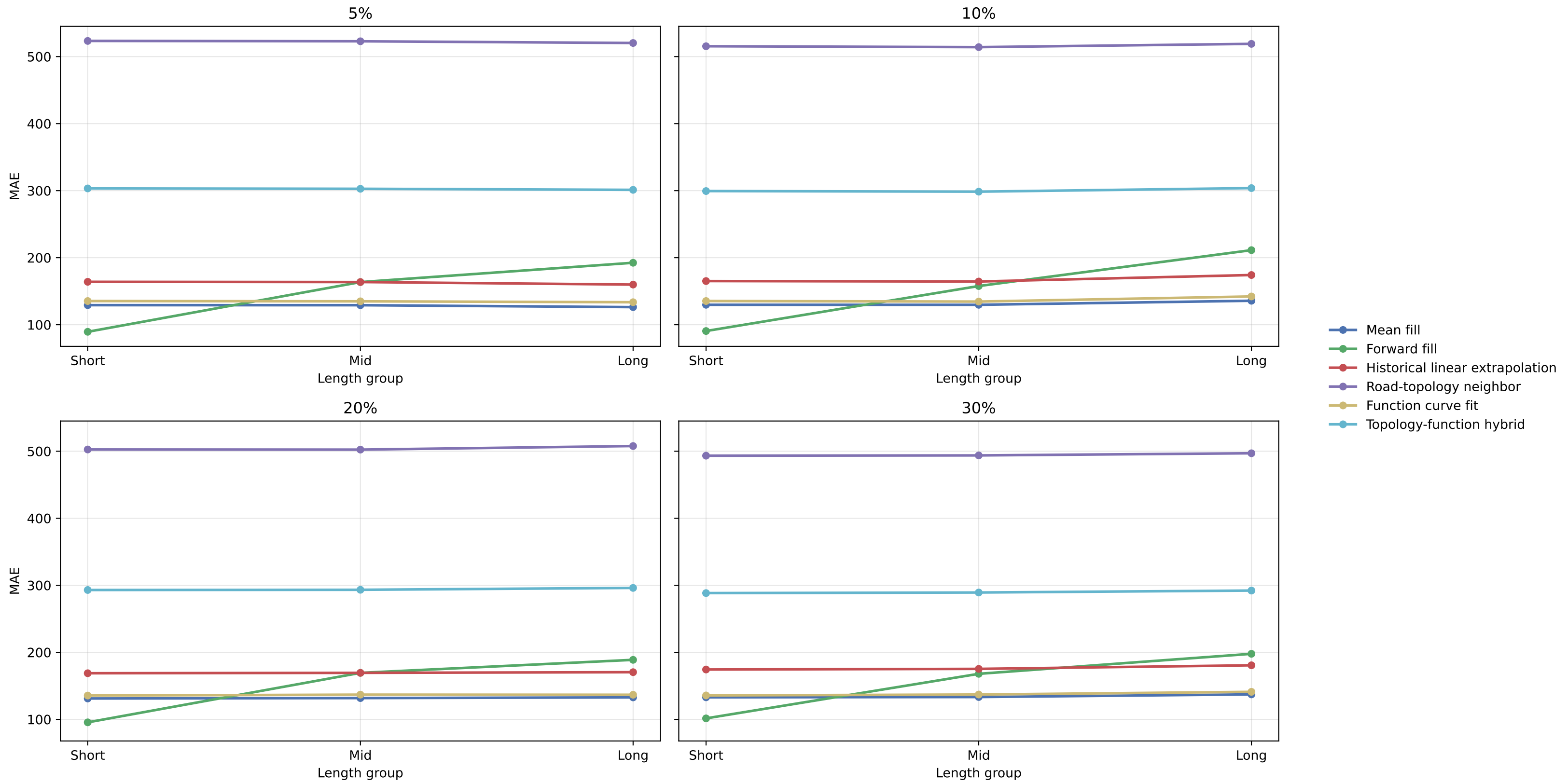
Node subset temporal outage MAE by Length Group
