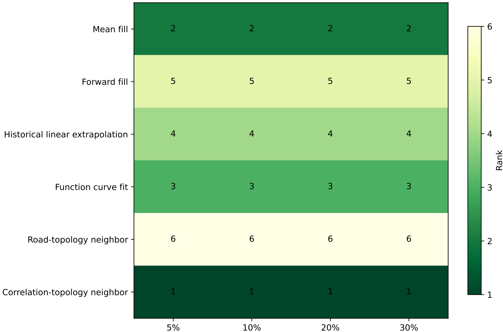
snh_mix RMSE Rank Heatmap
