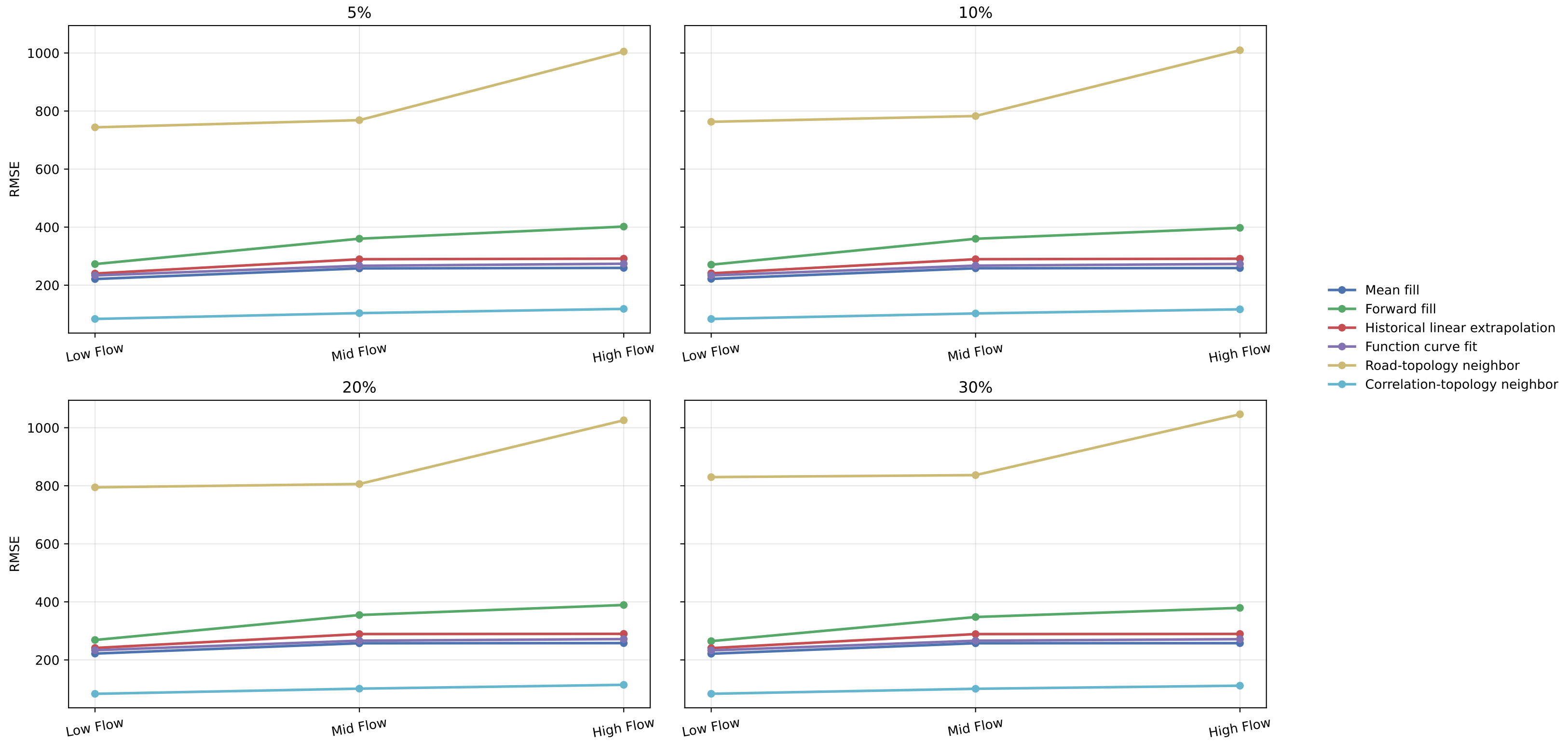
snh_mix RMSE by Flow Group and Method Rates: 5%, 10%, 20%, 30% Evaluation: masked-position imputation error
