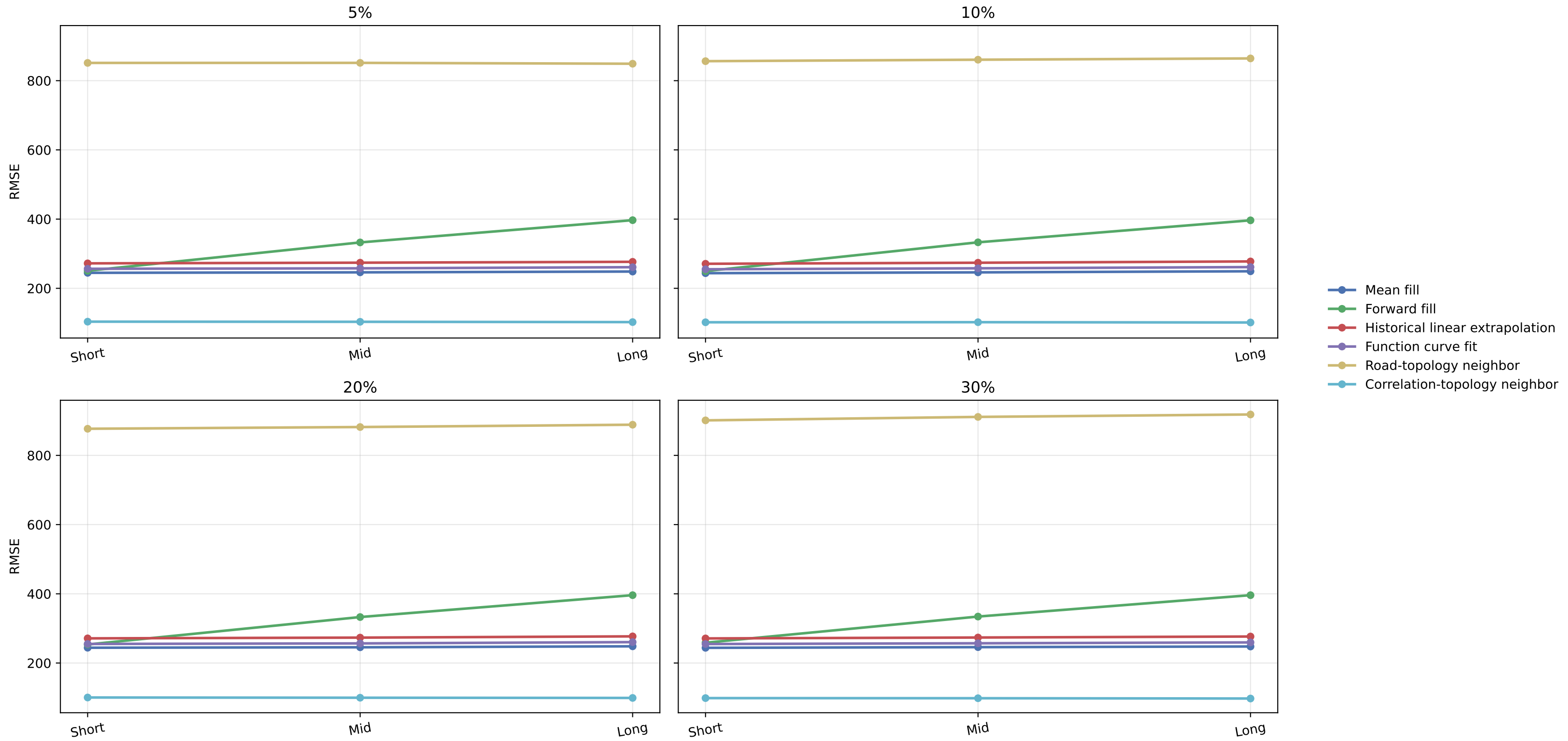
snh_mix RMSE by Length Group and Method Rates: 5%, 10%, 20%, 30% Evaluation: masked-position imputation error
