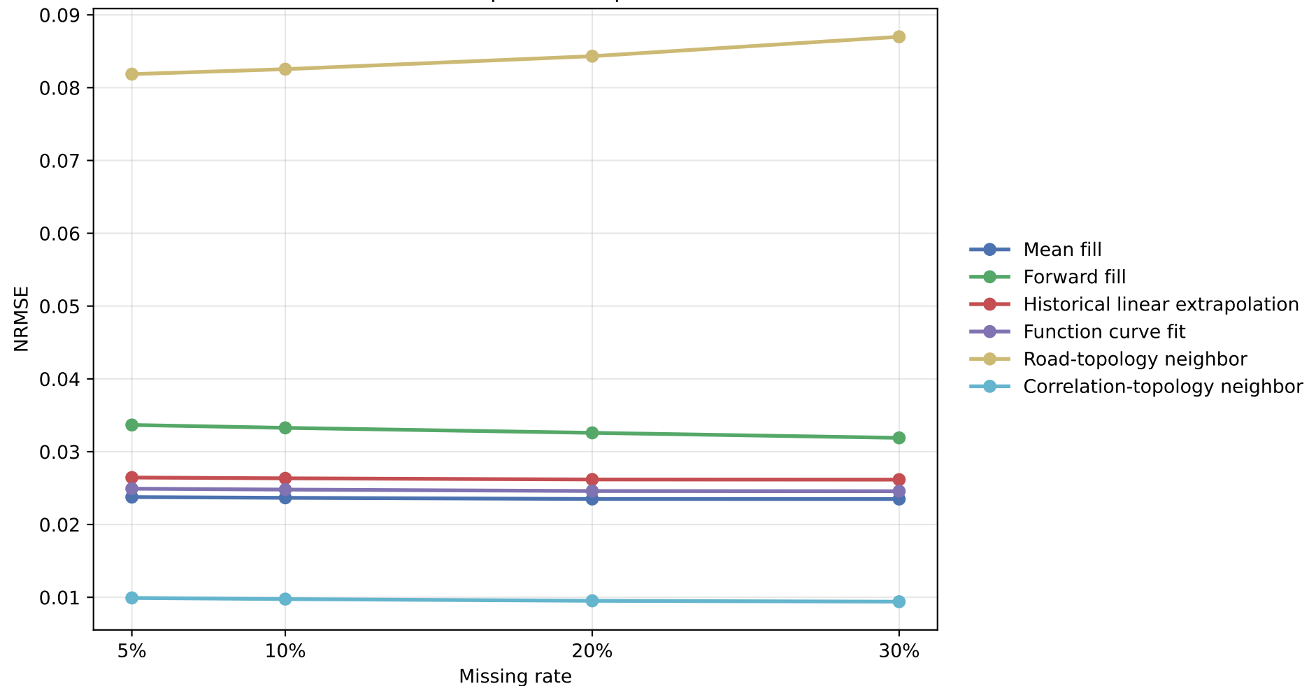
snh_mix NRMSE by Method Rates: 5%, 10%, 20%, 30% Evaluation: masked-position imputation error
