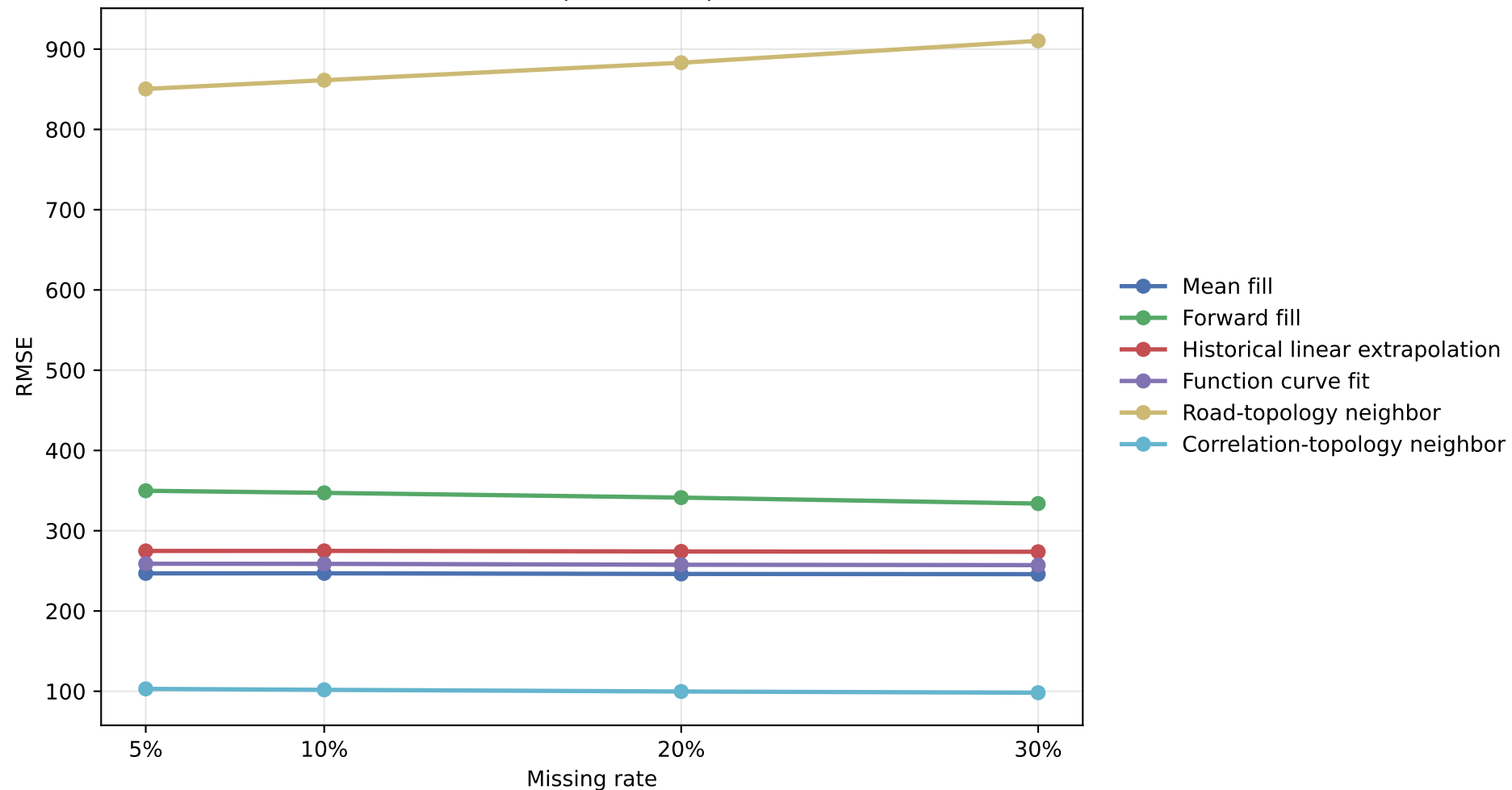
snh_mix RMSE by Method Rates: 5%, 10%, 20%, 30% Evaluation: masked-position imputation error
