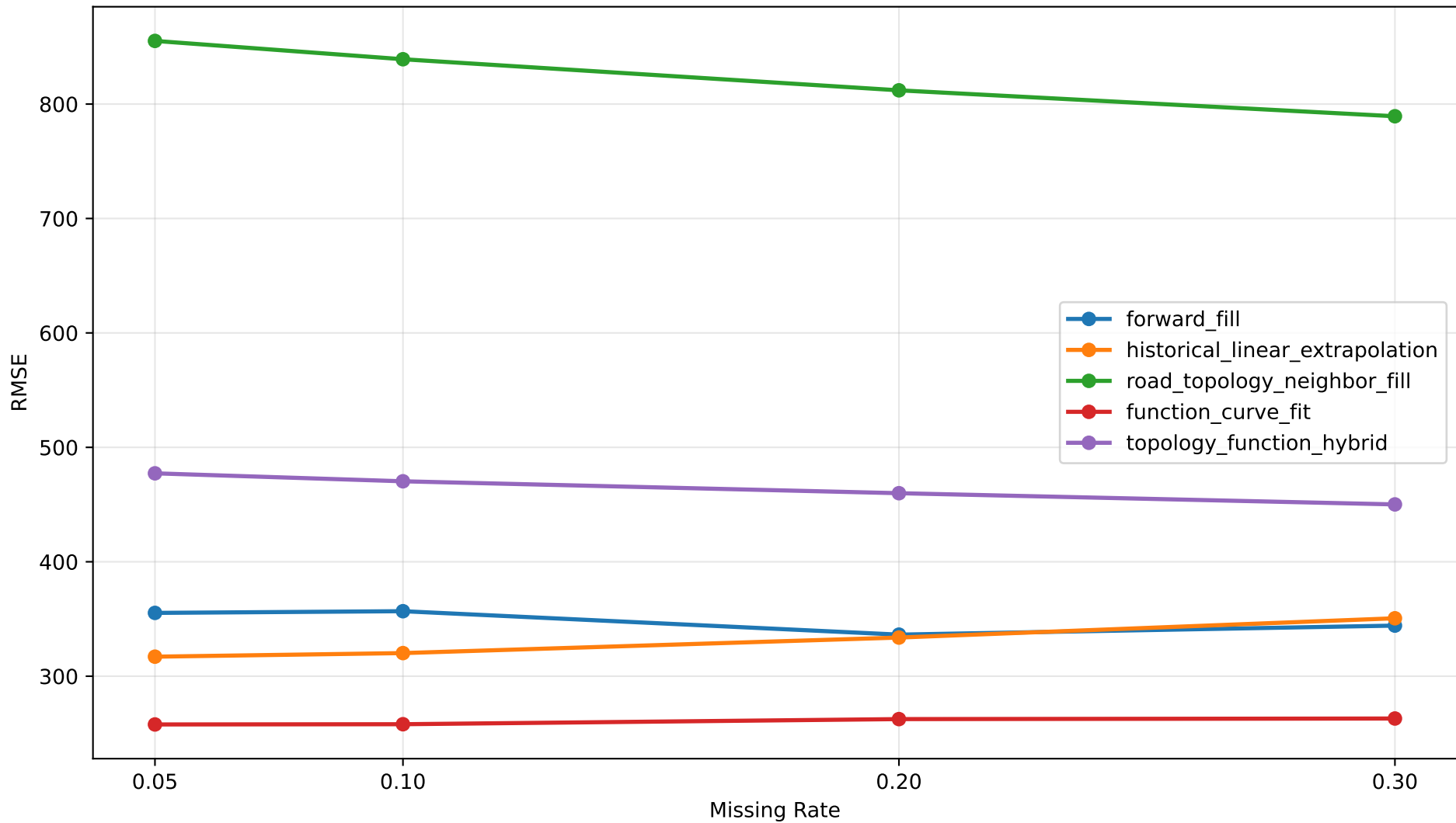
Structured Temporal Block RMSE by Method (Non-Zero Methods Only)
