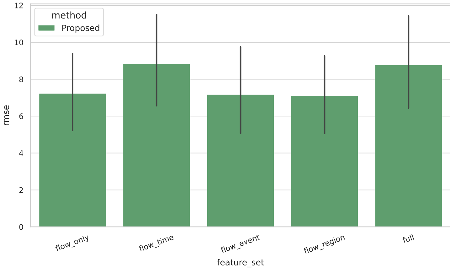
Feature Ablation
