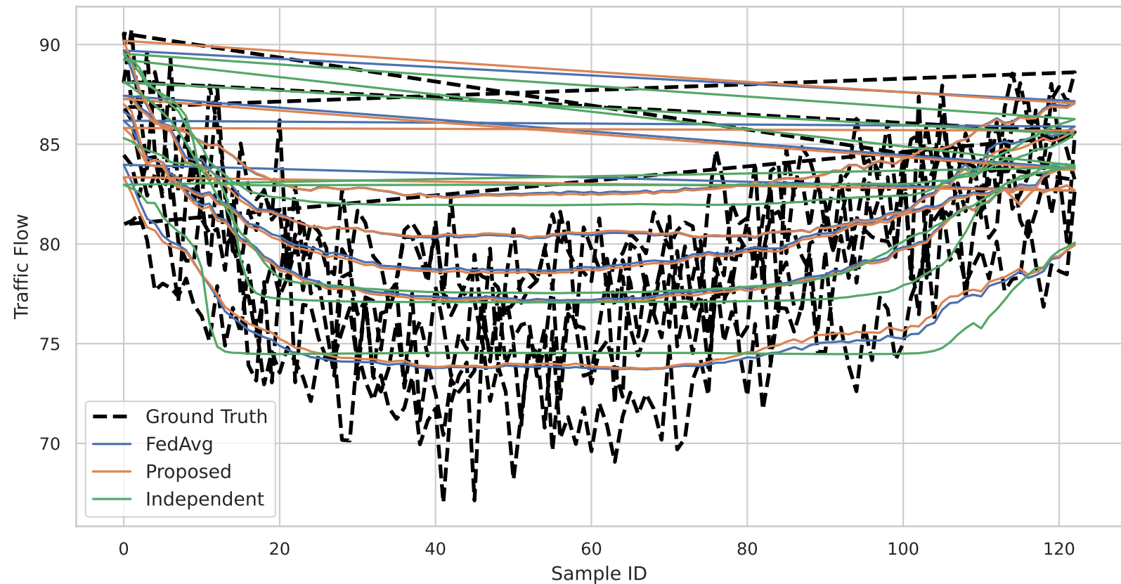
Main Prediction Comparison (Client 0)
