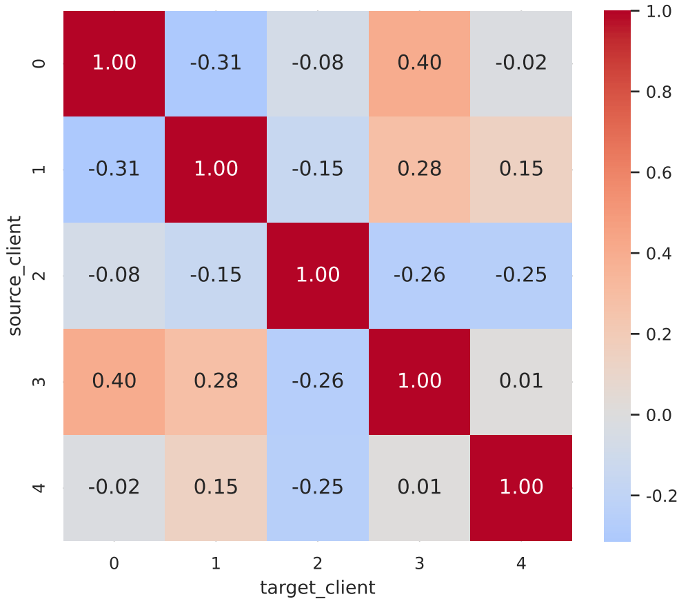
Client Correlation Matrix
