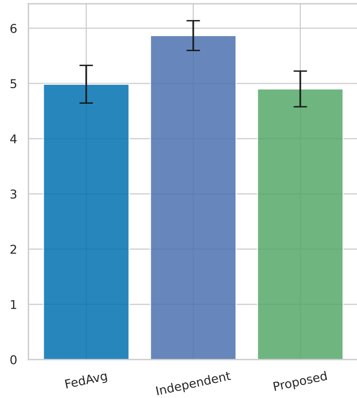
Multi-seed Mean \pm Std: MAE
