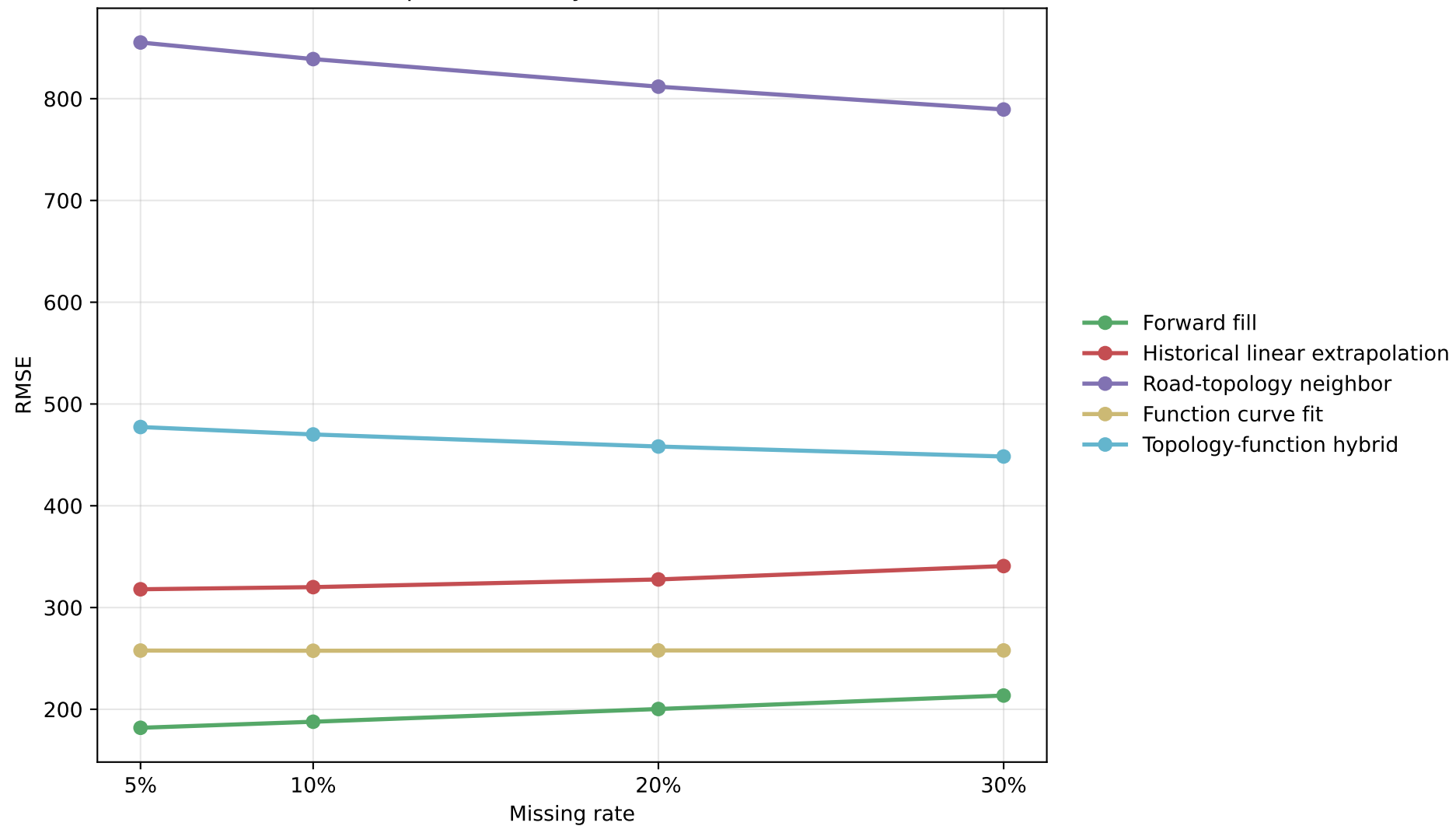
Global MCAR point RMSE by Method (Non-zero Zoom)
