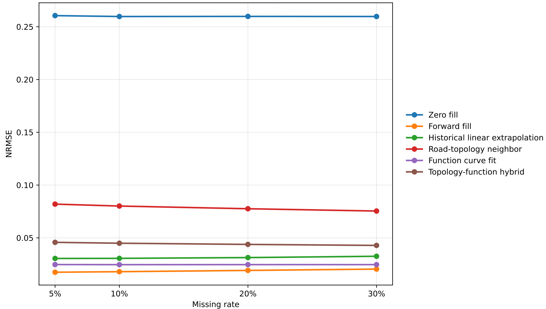
NRMSE by method across missing rates
