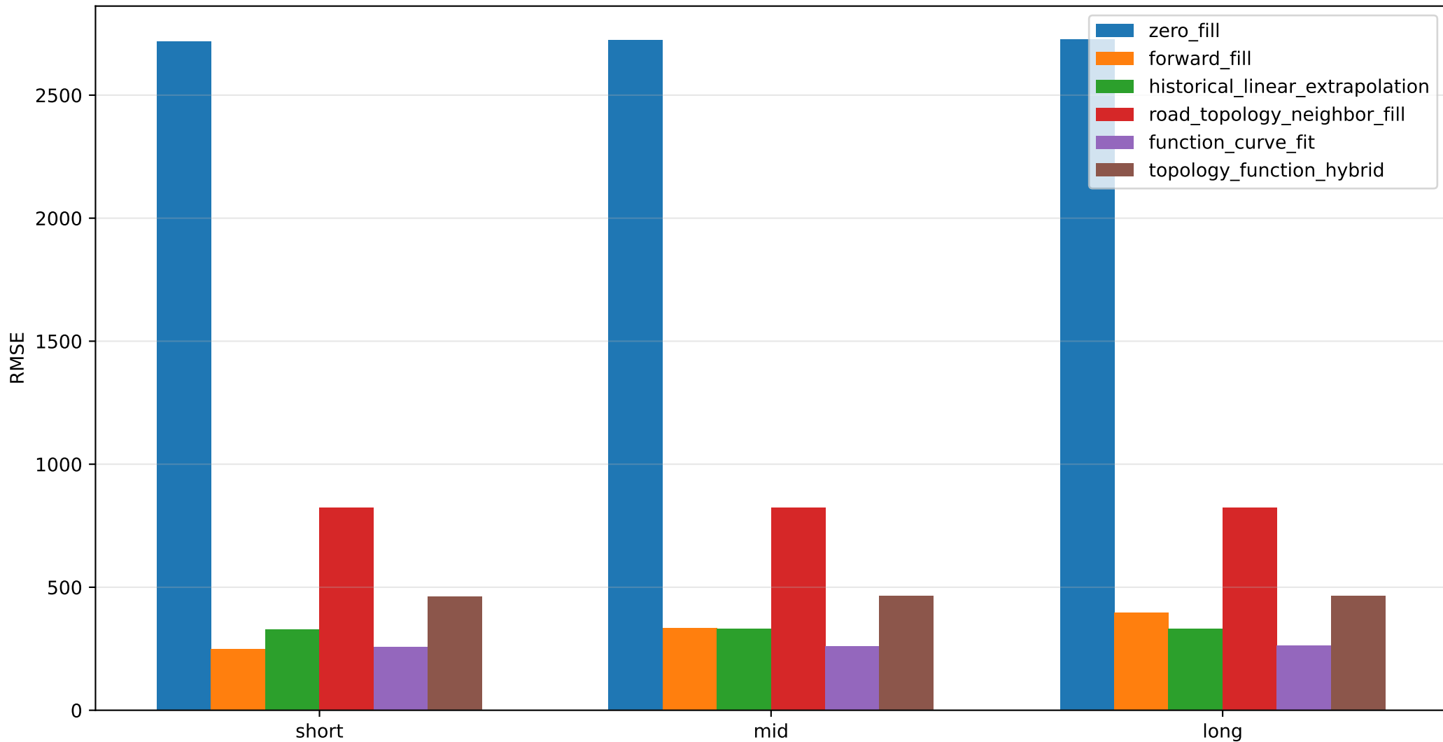
Structured Temporal Block RMSE by Length Group and Method
