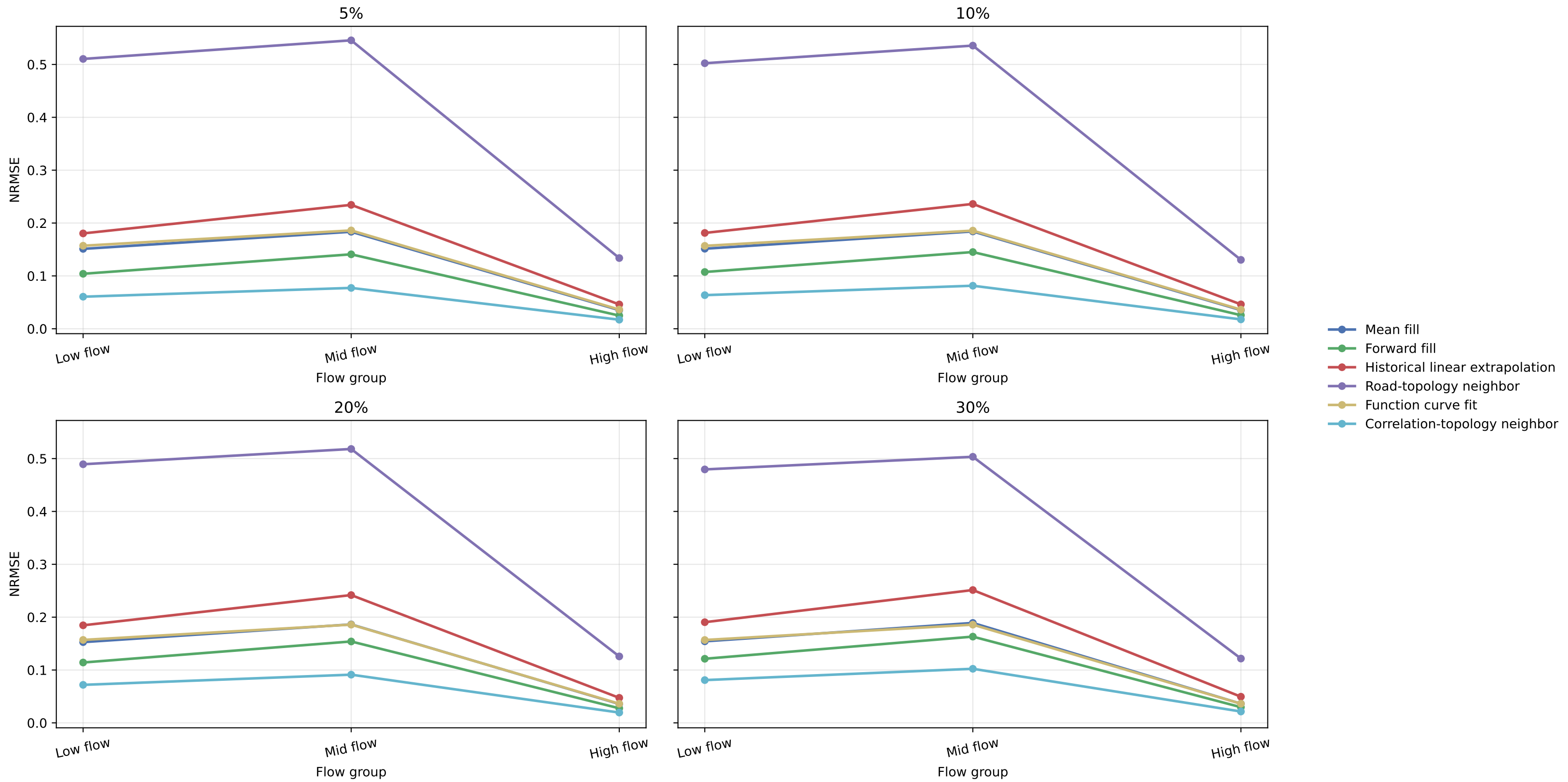
Global MCAR point NRMSE by Flow Group
