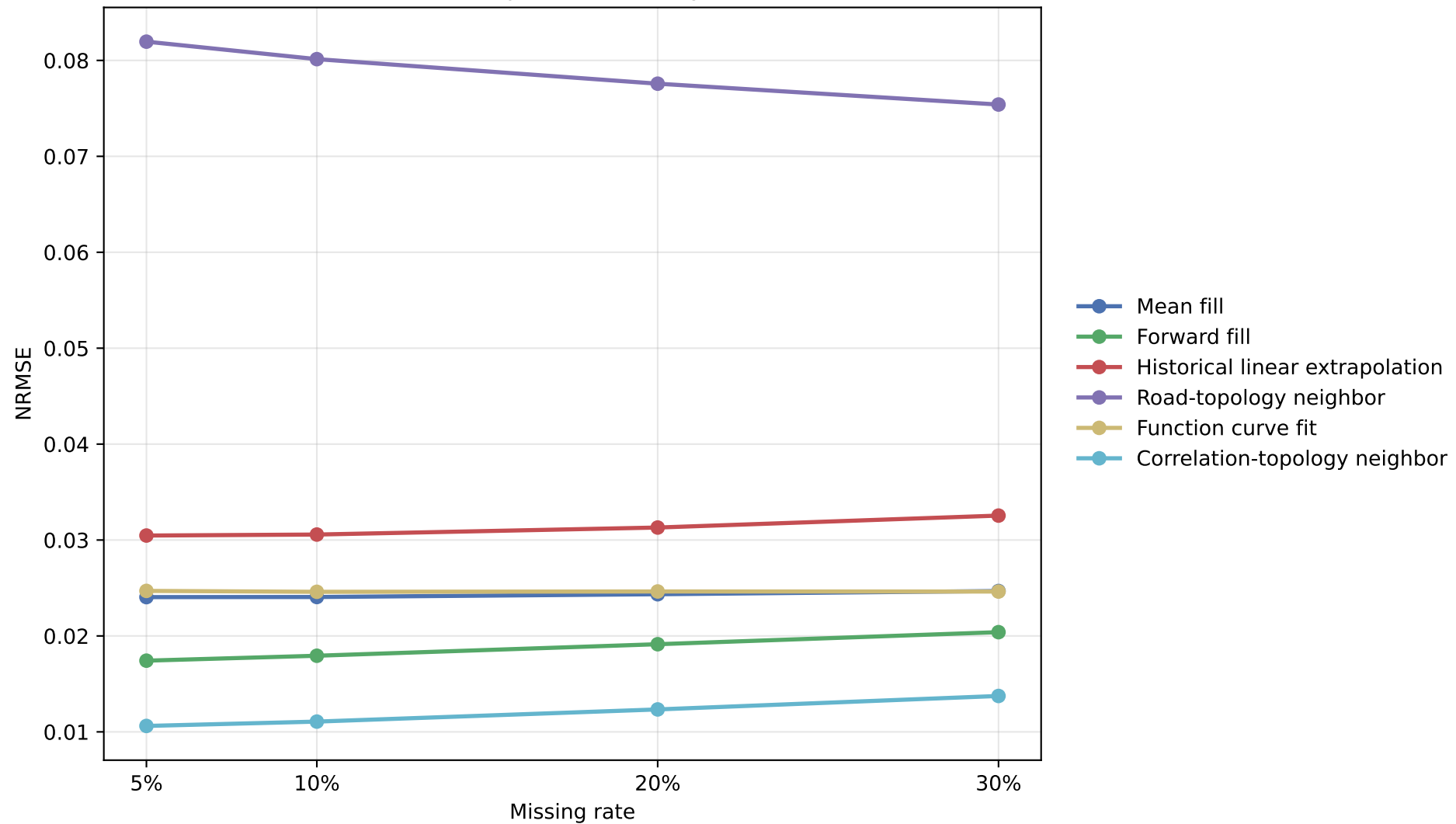
Global MCAR point NRMSE by Method
