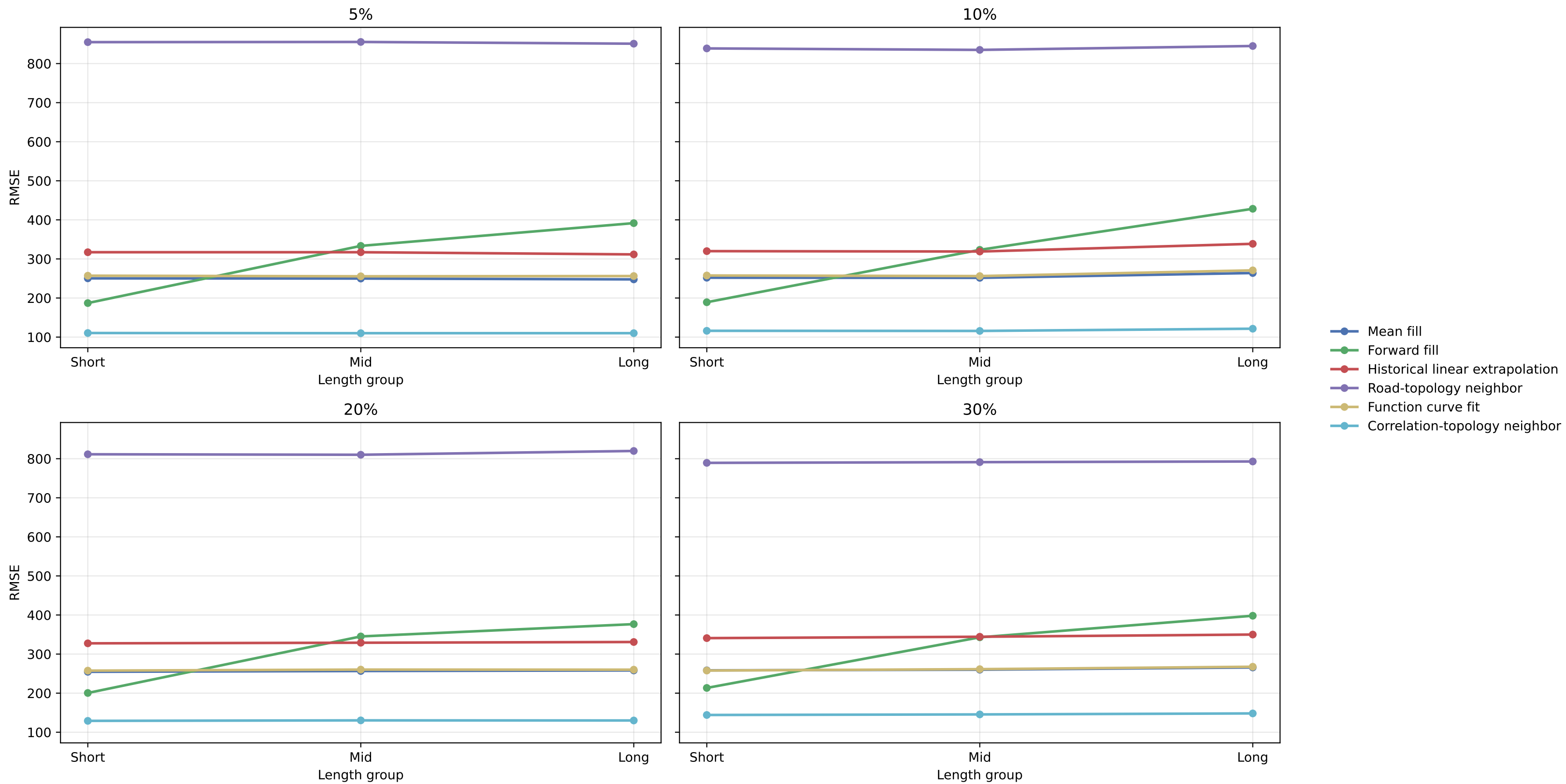
Node subset temporal outage RMSE by Length Group
