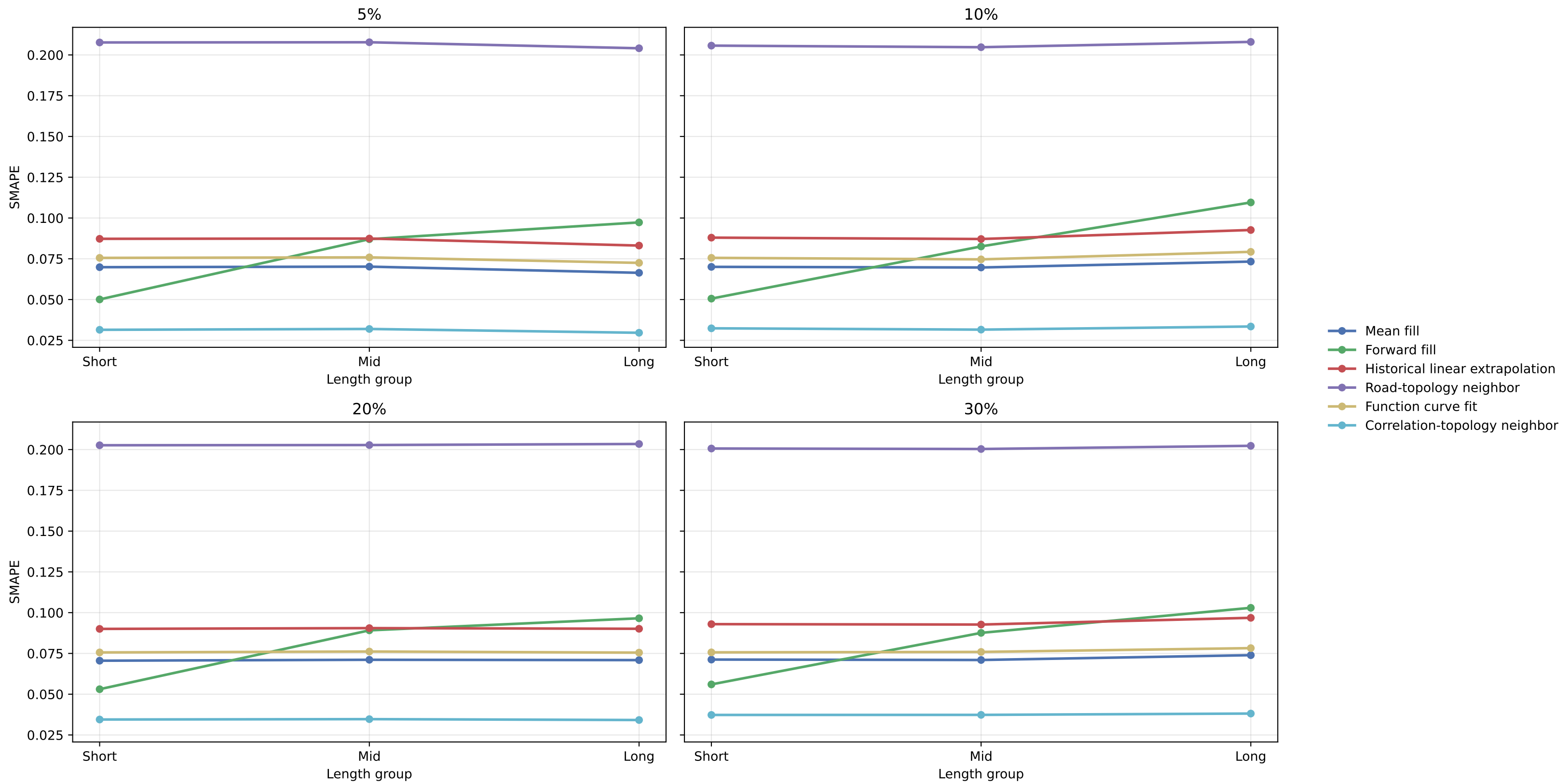
Node subset temporal outage SMAPE by Length Group
