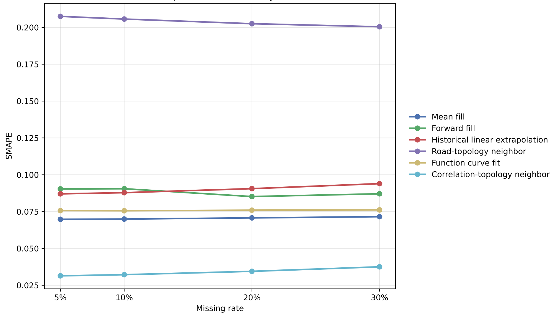
Node temporal block SMAPE by Method
