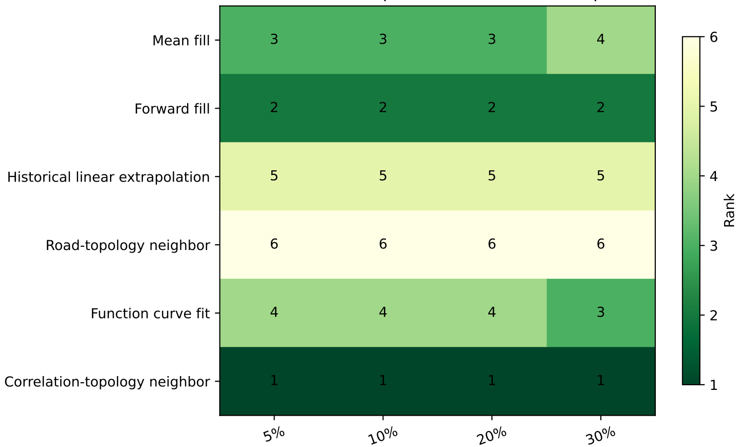
Global MCAR point RMSE Rank Heatmap
