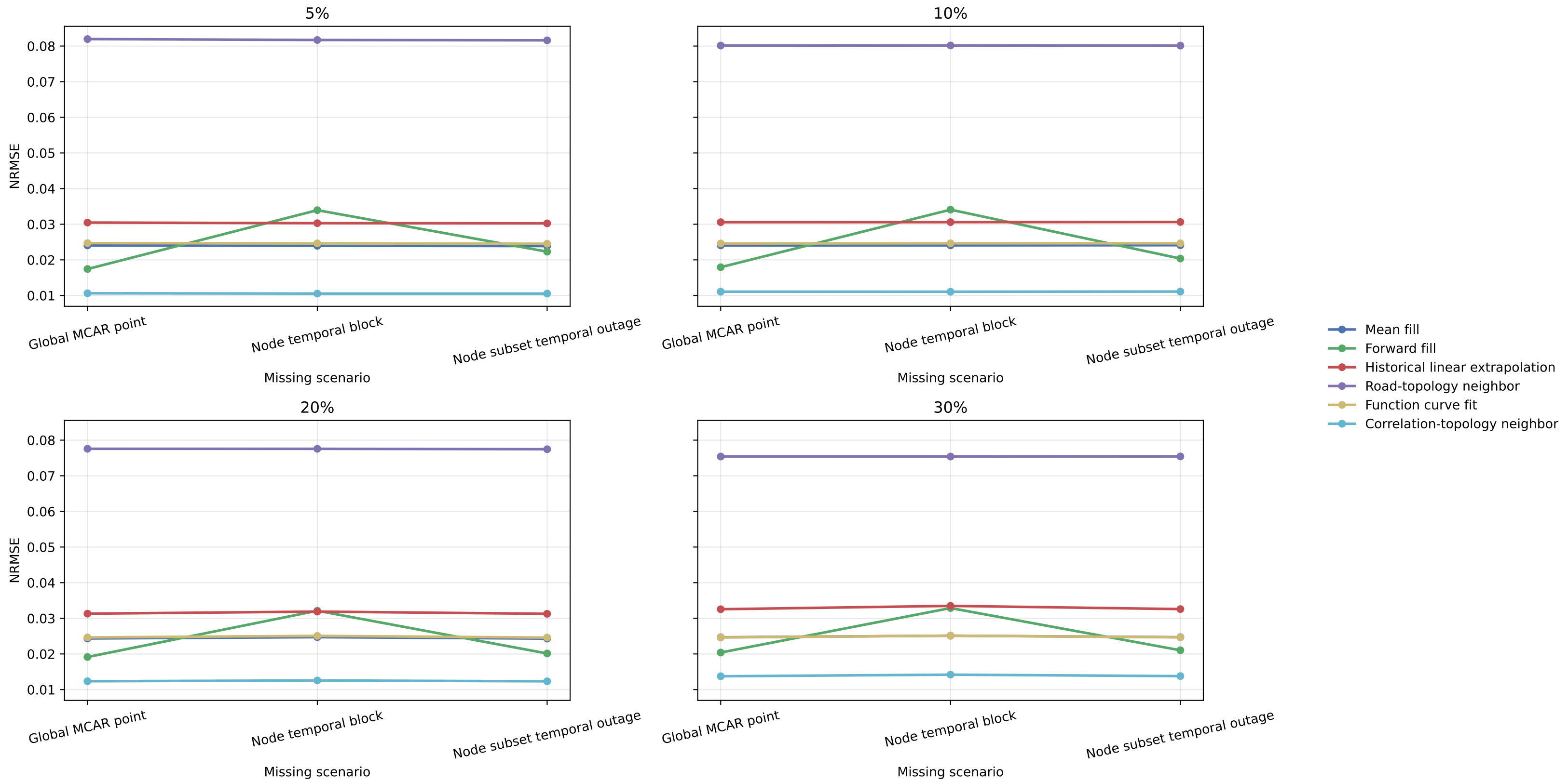
Scenario Comparison NRMSE by Method
