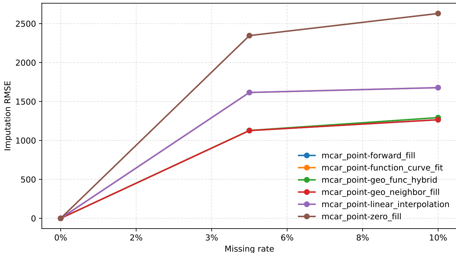
Imputation RMSE under Artificial Missing Rates Real Data (Geo + Func)
