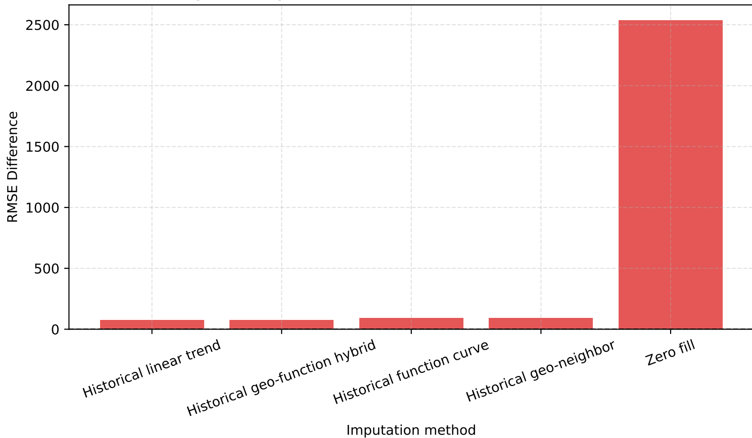
Single missing rate = 5%: RMSE delta relative to forward fill
