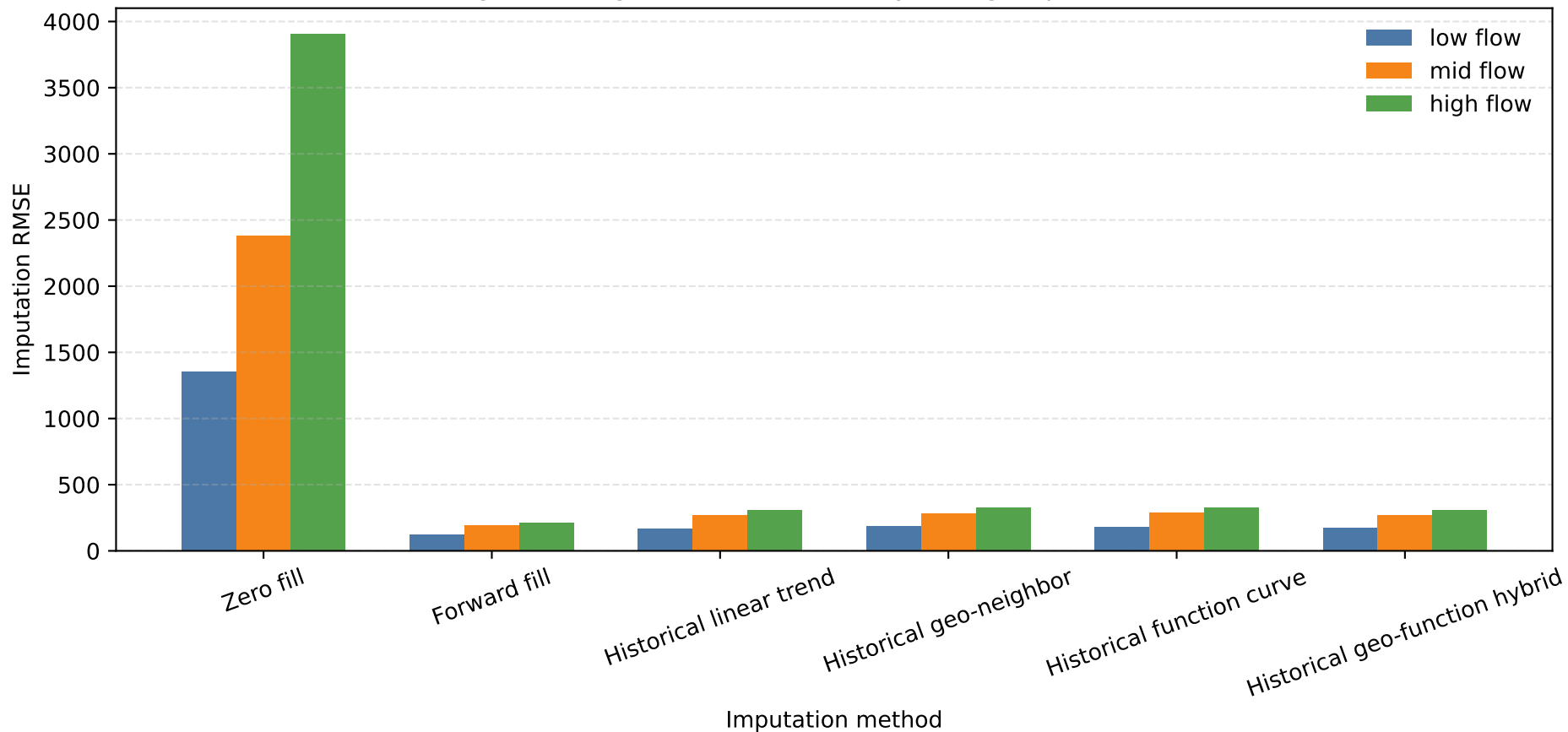
Single missing rate = 5%: RMSE by flow group and method
