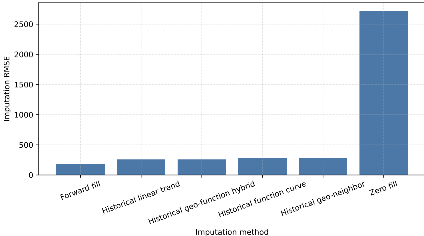
Single missing rate = 5%: Imputation RMSE by method Full Intersection-stage Real Data, Historical Causal Setting
