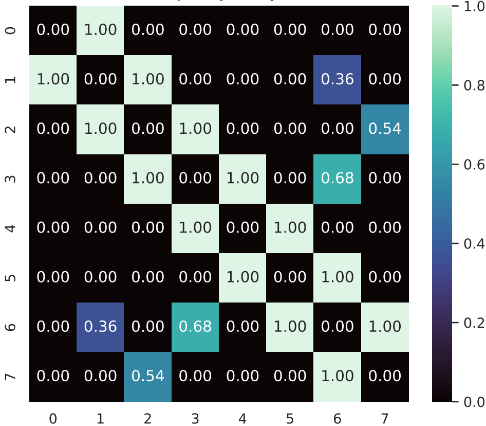
Base Graph Adjacency Matrix
