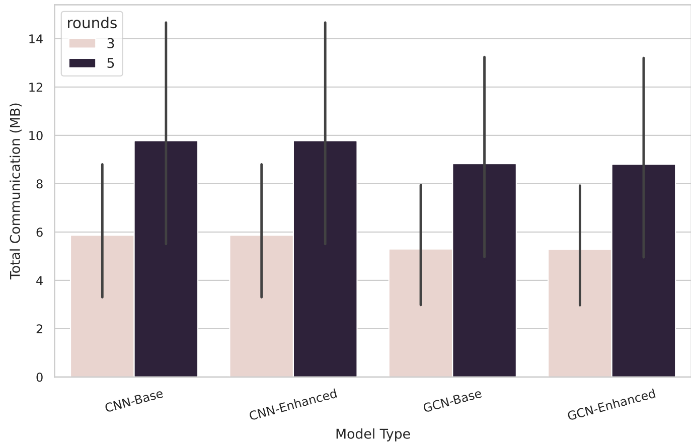
Communication Cost
