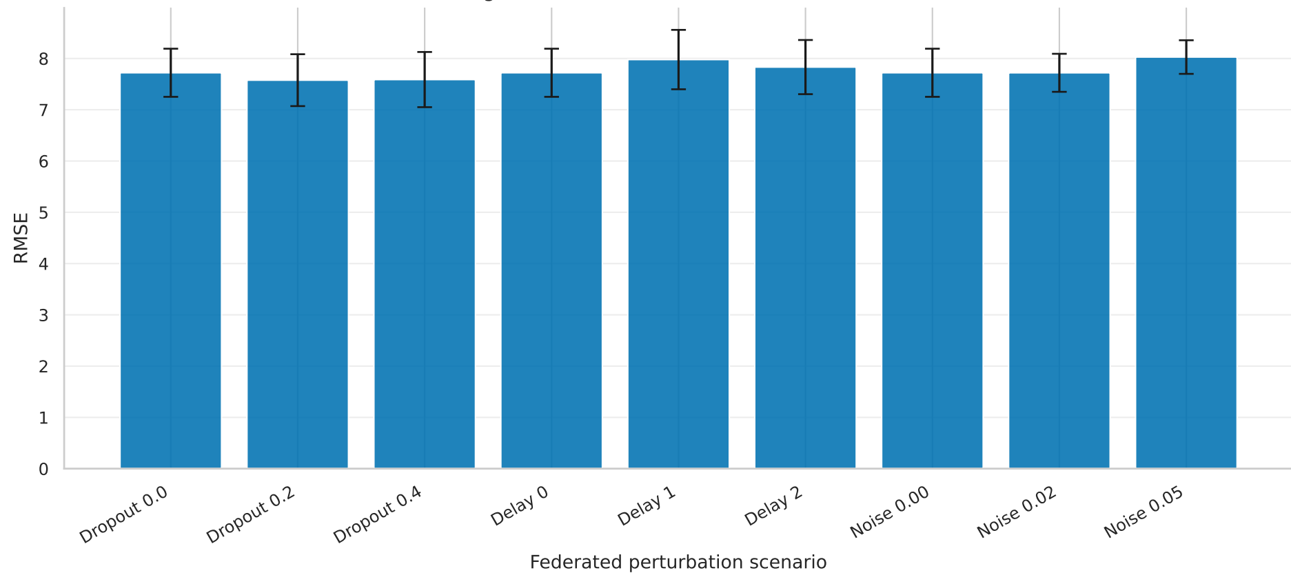
FedAvg Robustness under Federated Perturbations
