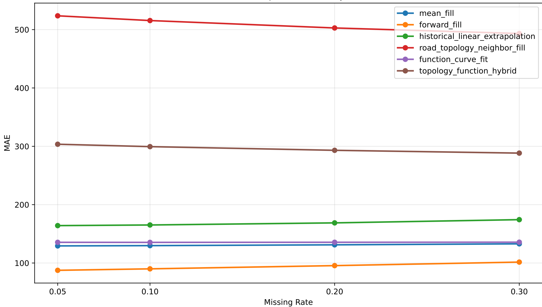
Global MCAR Imputation MAE by Method
