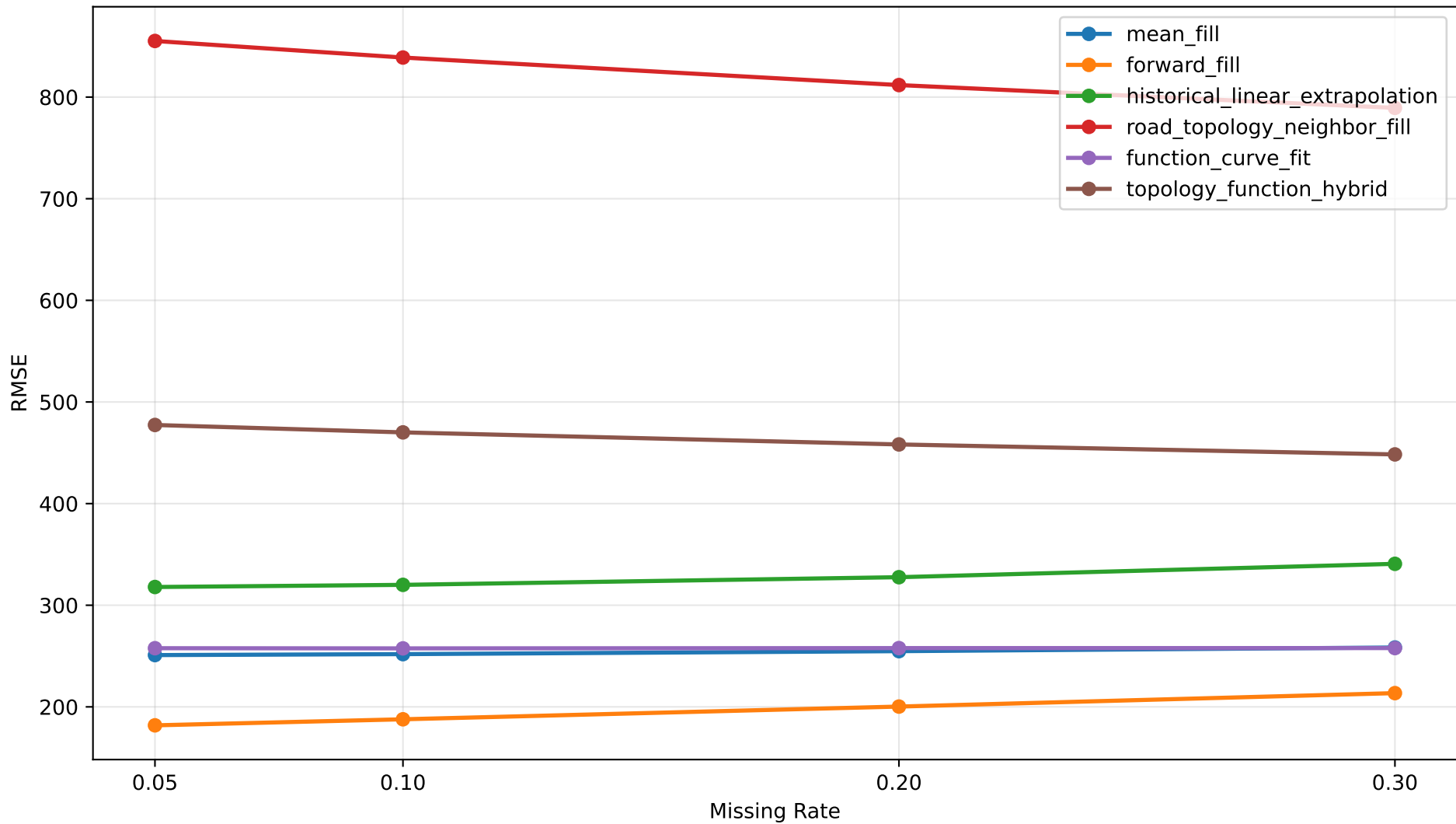
Global MCAR Imputation RMSE by Method
